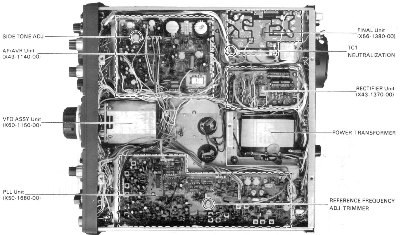
Bottom View
